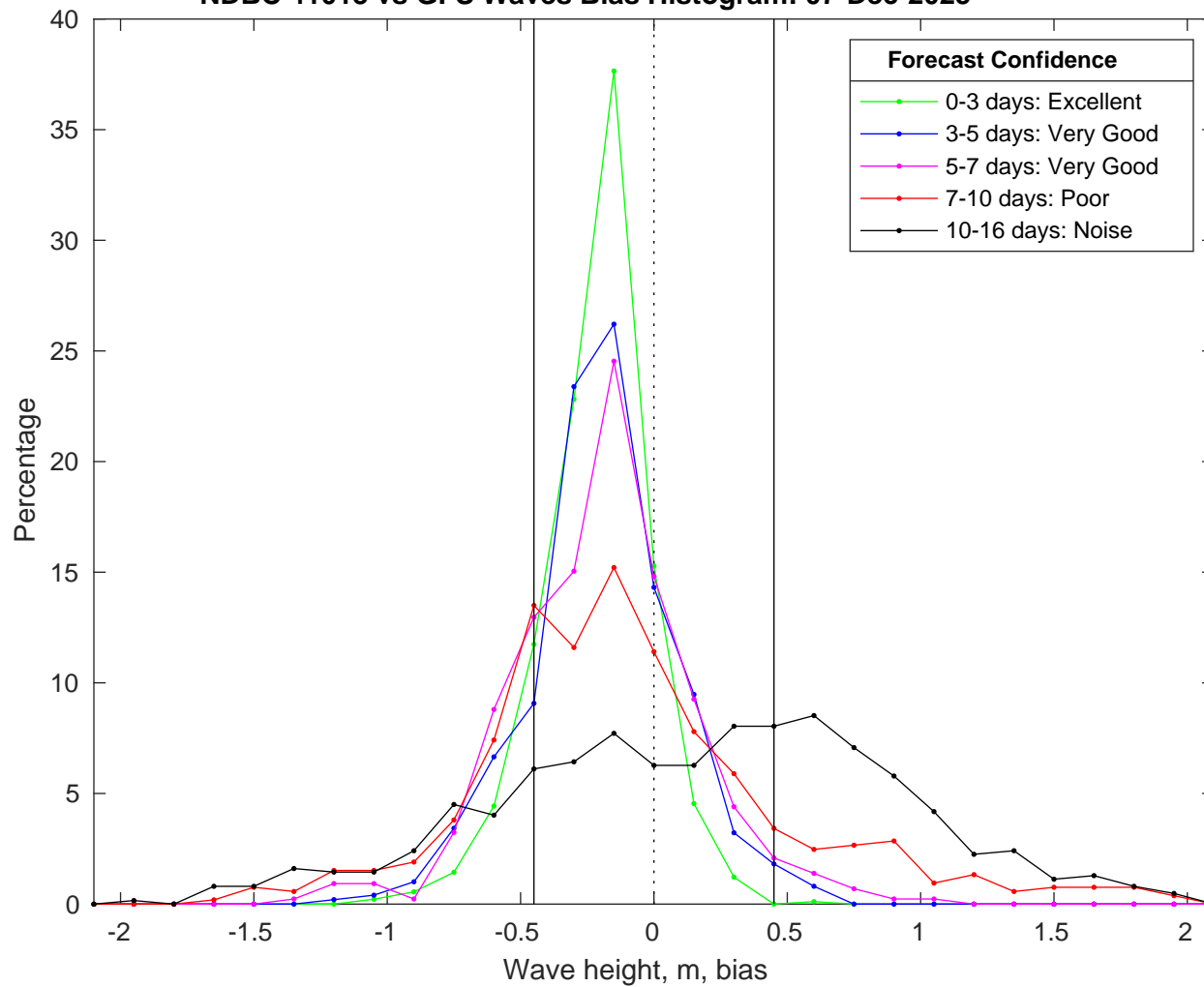
NDBC 41013 vs GFS Waves Bias Histogram: 07-Dec-2025
