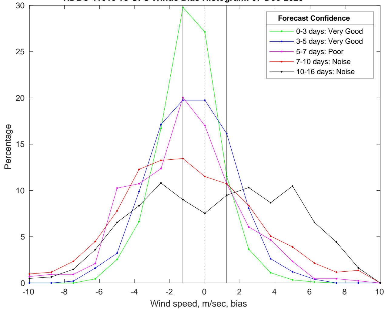
NDBC 41013 vs GFS Winds Bias Histogram: 07-Dec-2025
