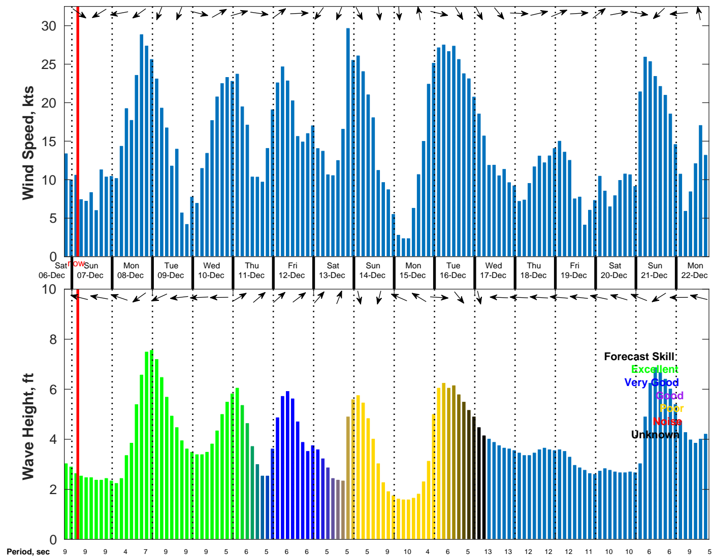
Wind & Wave Forecast for NDBC 41013 from 06-Dec-2025 19:00:00 to 22-Dec-2025 19:00:00
