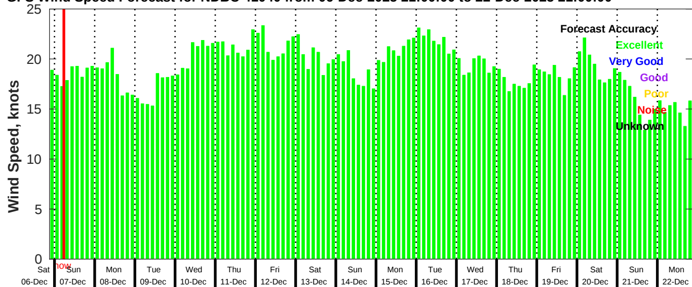
GFS Wind Speed Forecast for NDBC 41040 from 06-Dec-2025 21:00:00 to 22-Dec-2025 21:00:00
