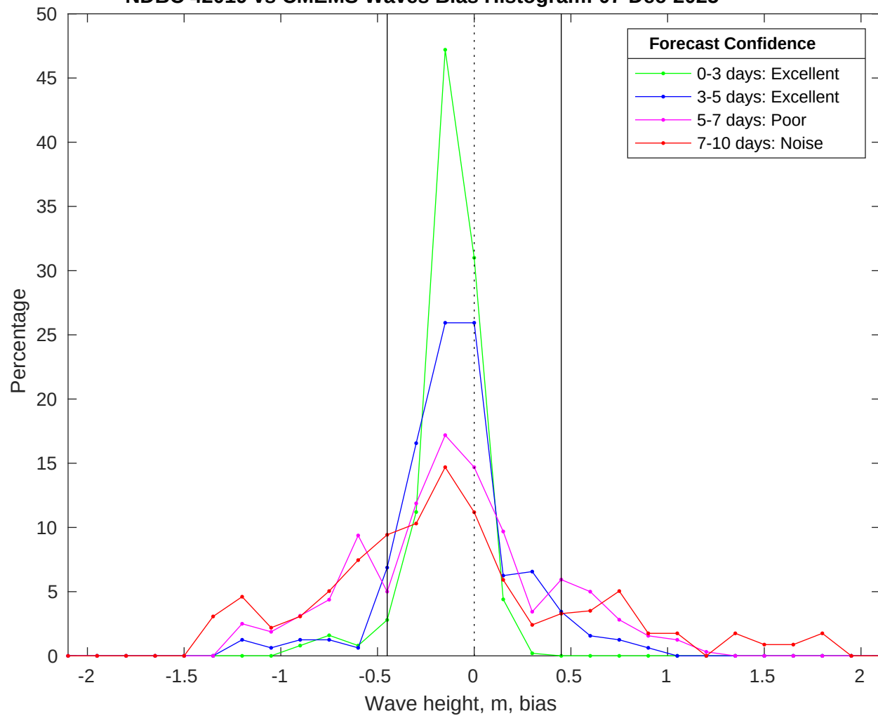
NDBC 42019 vs CMEMS Waves Bias Histogram: 07-Dec-2025
