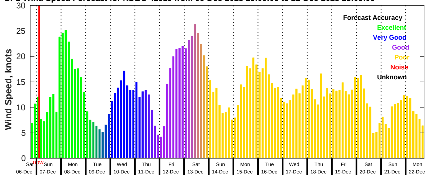
GFS Wind Speed Forecast for NDBC 42019 from 06-Dec-2025 18:00:00 to 22-Dec-2025 18:00:00
