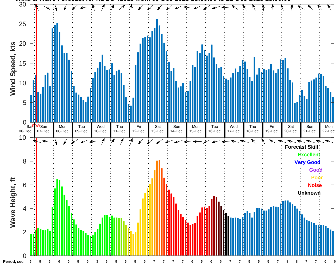
Wind & Wave Forecast for NDBC 42019 from 06-Dec-2025 18:00:00 to 22-Dec-2025 18:00:00
