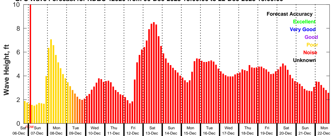
GFS Wave Forecast for NDBC 42020 from 06-Dec-2025 18:00:00 to 22-Dec-2025 18:00:00
