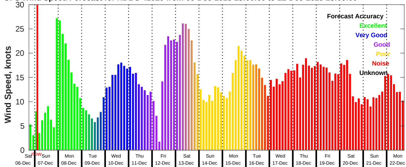
GFS Wind Speed Forecast for NDBC 42020 from 06-Dec-2025 18:00:00 to 22-Dec-2025 18:00:00
