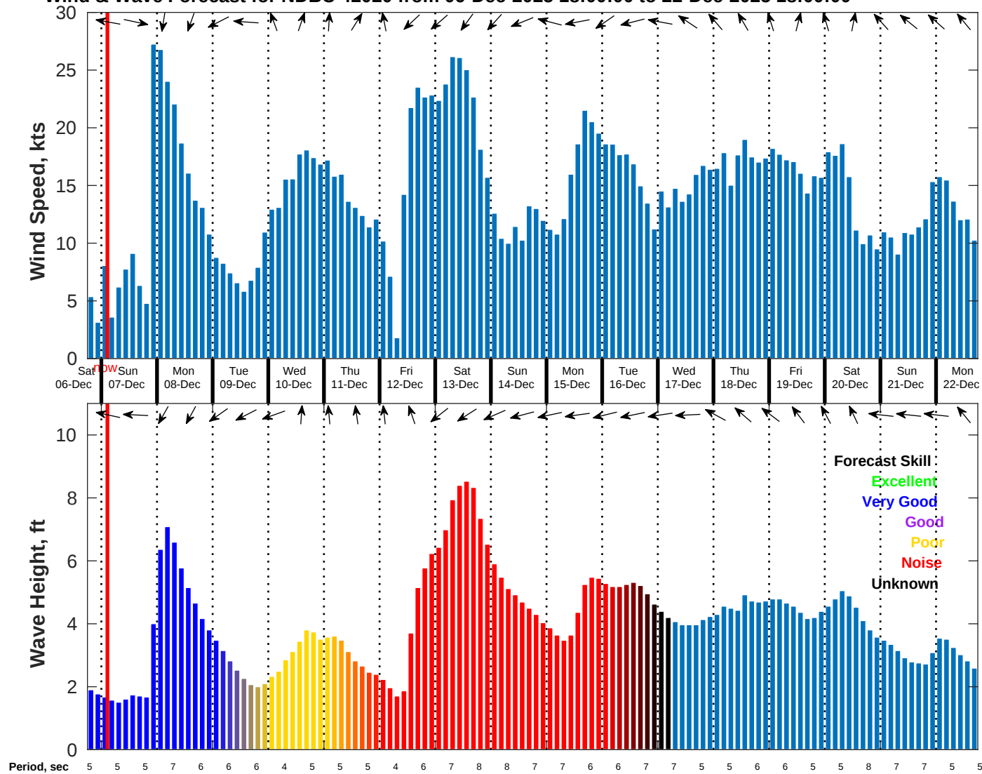
Wind & Wave Forecast for NDBC 42020 from 06-Dec-2025 18:00:00 to 22-Dec-2025 18:00:00
