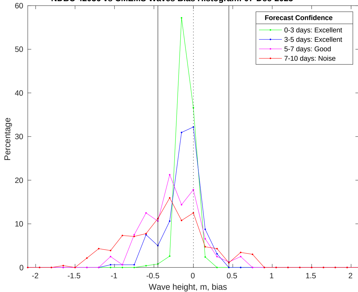
NDBC 42036 vs CMEMS Waves Bias Histogram: 07-Dec-2025
