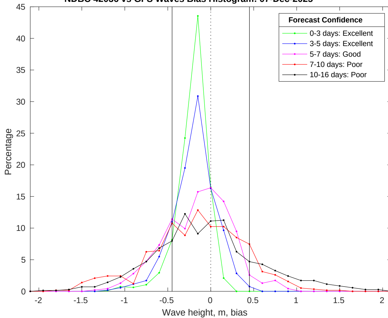
NDBC 42036 vs GFS Waves Bias Histogram: 07-Dec-2025
