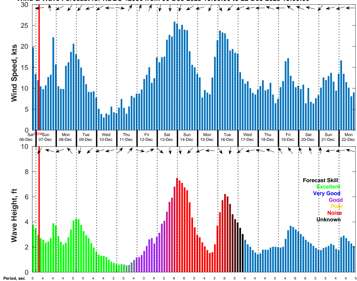
Wind & Wave Forecast for NDBC 42036 from 06-Dec-2025 19:00:00 to 22-Dec-2025 19:00:00
