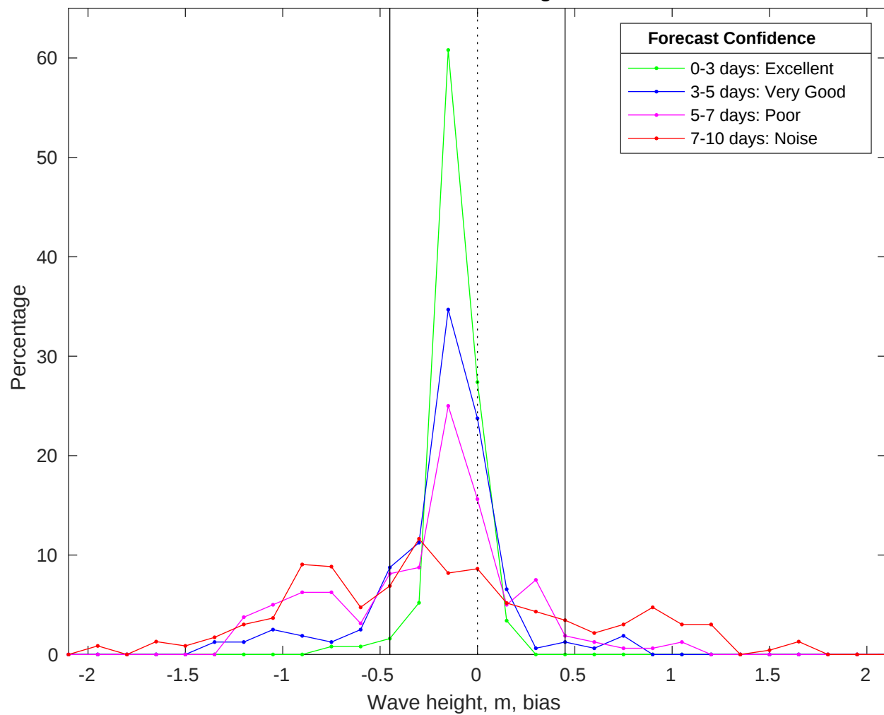
NDBC 42040 vs CMEMS Waves Bias Histogram: 07-Dec-2025
