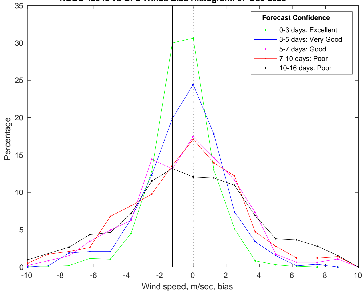
NDBC 42040 vs GFS Winds Bias Histogram: 07-Dec-2025
