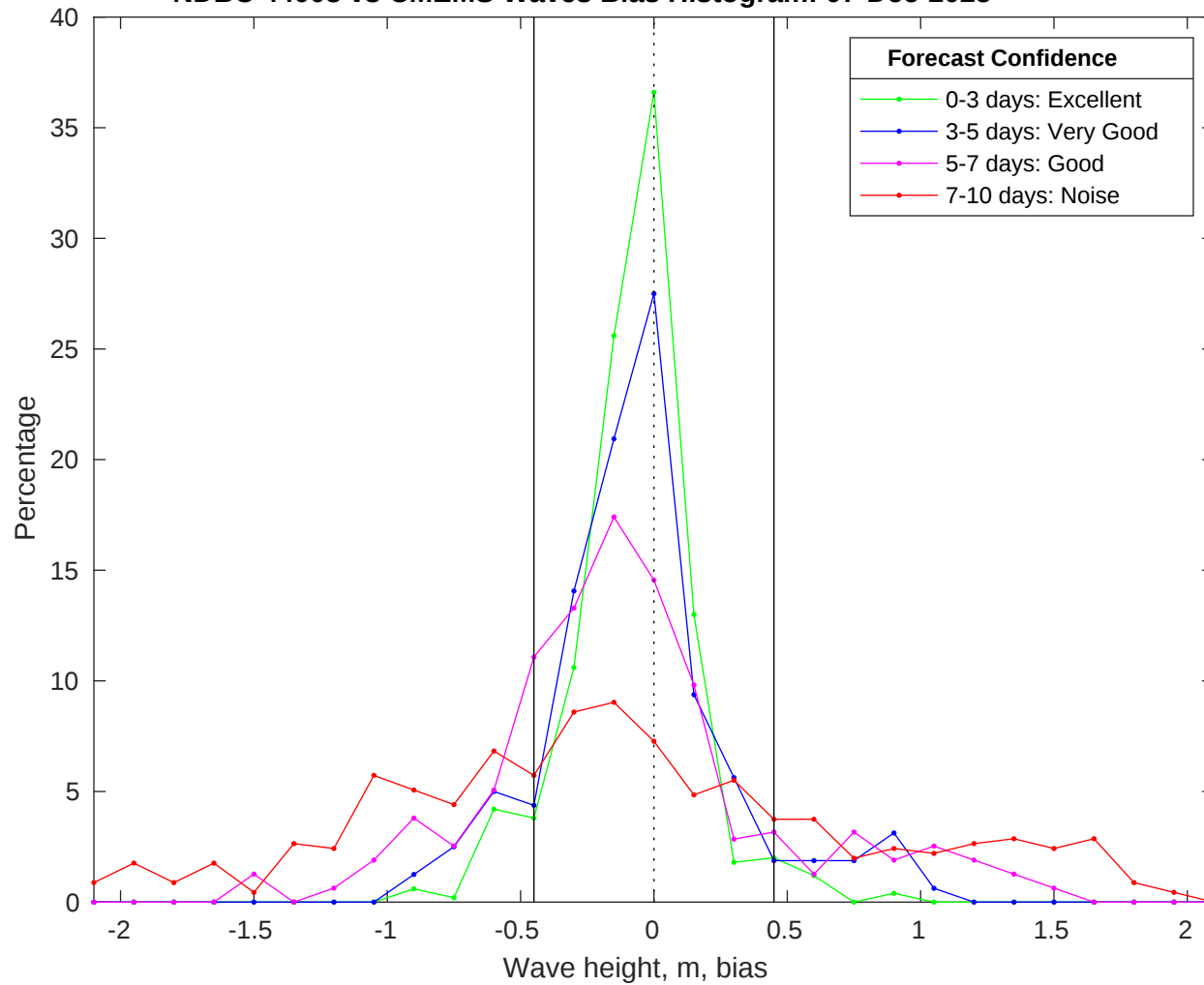
NDBC 44008 vs CMEMS Waves Bias Histogram: 07-Dec-2025
