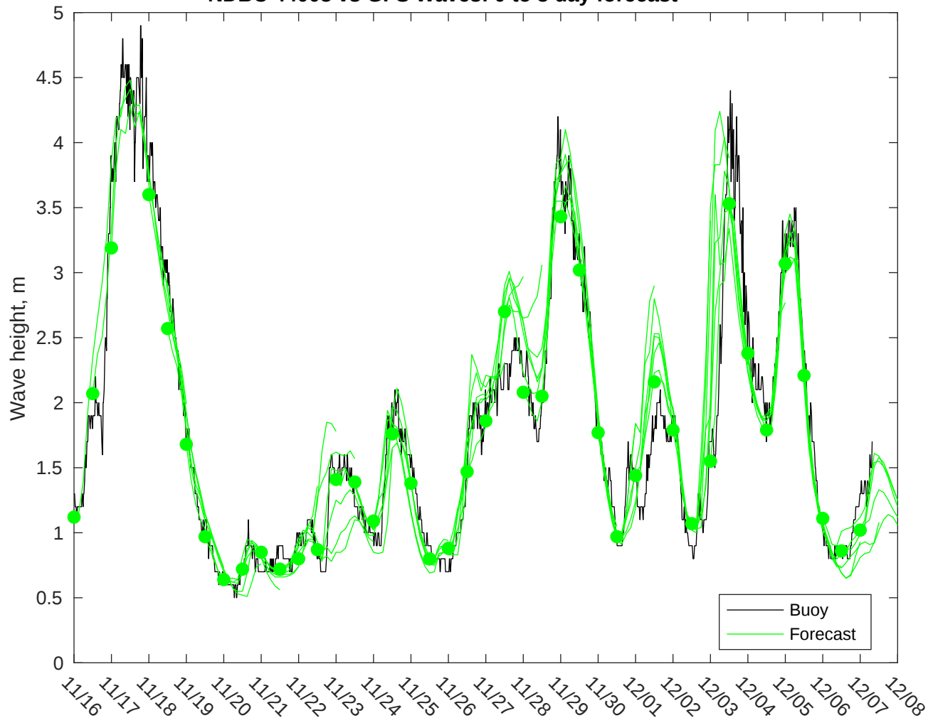
NDBC 44008 vs GFS Waves: 0 to 3 day forecast
