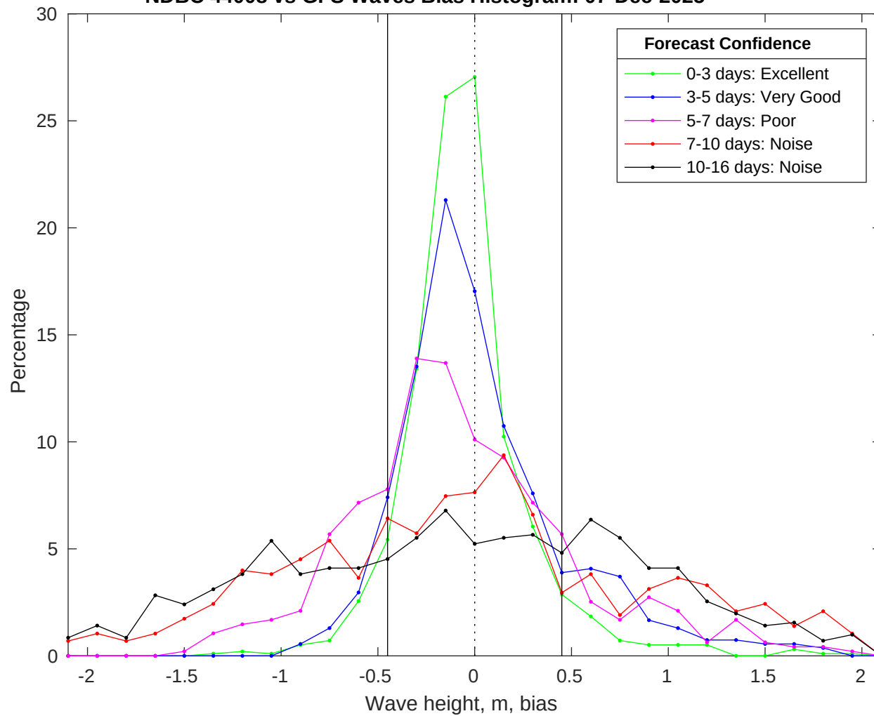
NDBC 44008 vs GFS Waves Bias Histogram: 07-Dec-2025
