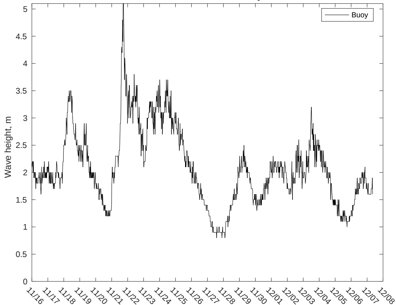
NDBC 46011 vs CMEMS Waves: 10 to 16 day forecast
