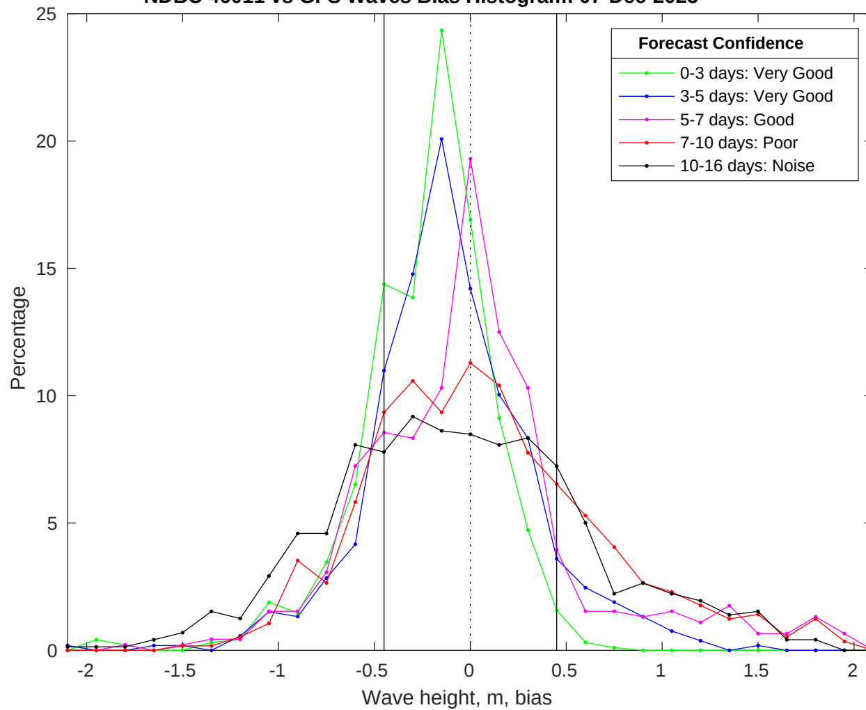
NDBC 46011 vs GFS Waves Bias Histogram: 07-Dec-2025
