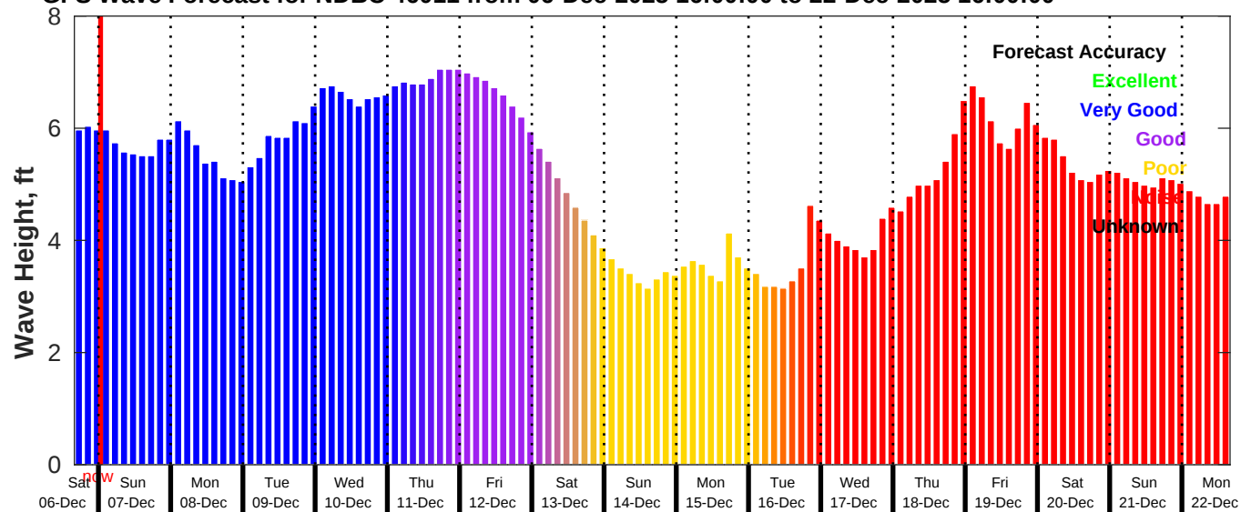
GFS Wave Forecast for NDBC 46011 from 06-Dec-2025 16:00:00 to 22-Dec-2025 16:00:00
