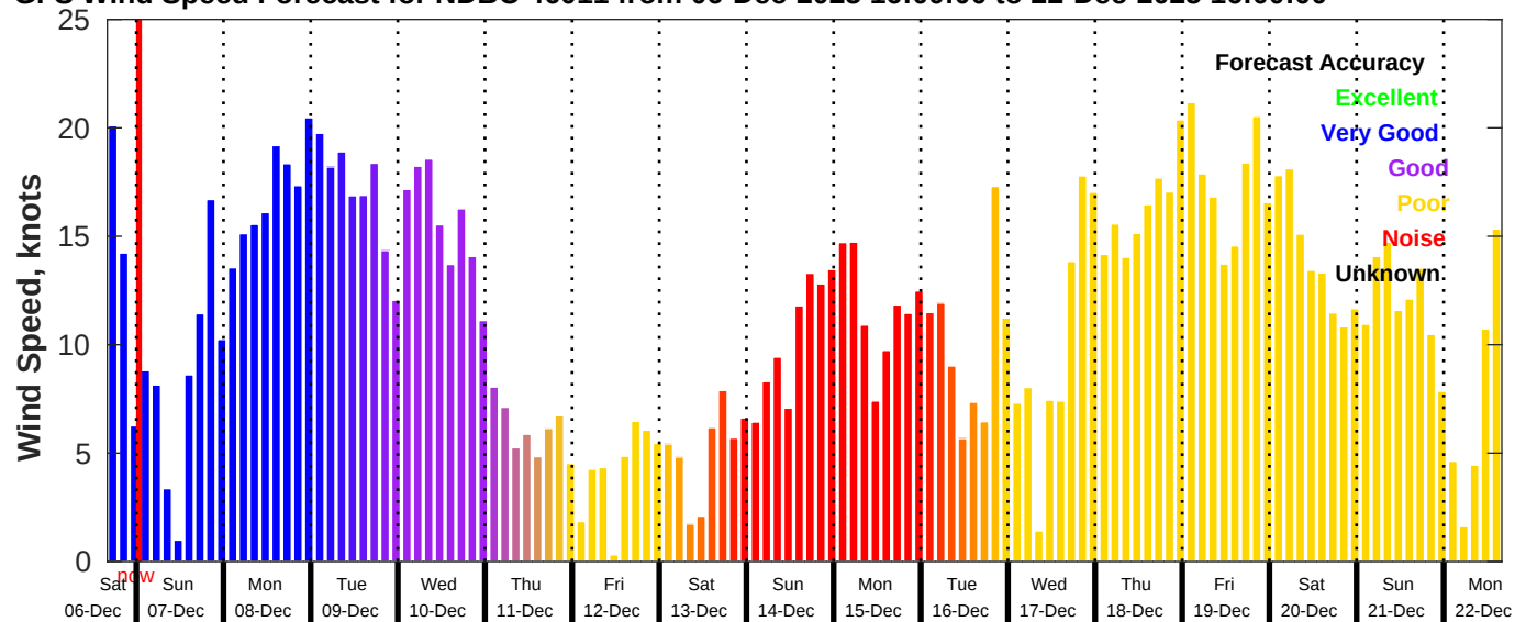
GFS Wind Speed Forecast for NDBC 46011 from 06-Dec-2025 16:00:00 to 22-Dec-2025 16:00:00
