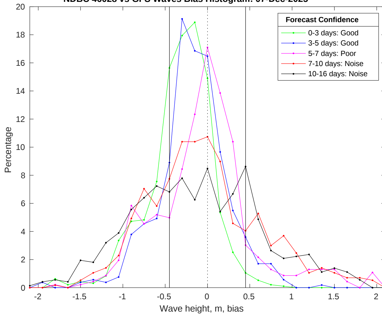
NDBC 46028 vs GFS Waves Bias Histogram: 07-Dec-2025
