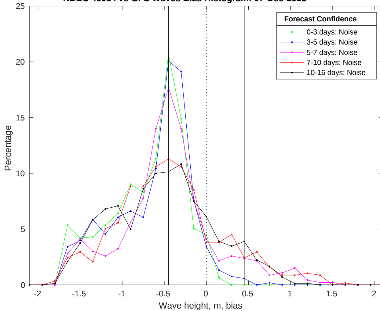
NDBC 46054 vs GFS Waves Bias Histogram: 07-Dec-2025
