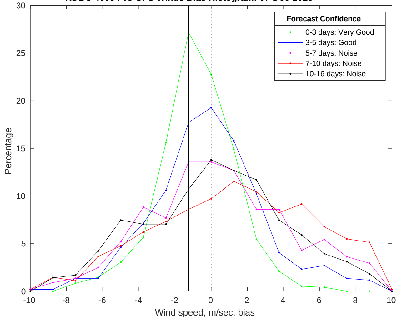
NDBC 46054 vs GFS Winds Bias Histogram: 07-Dec-2025
