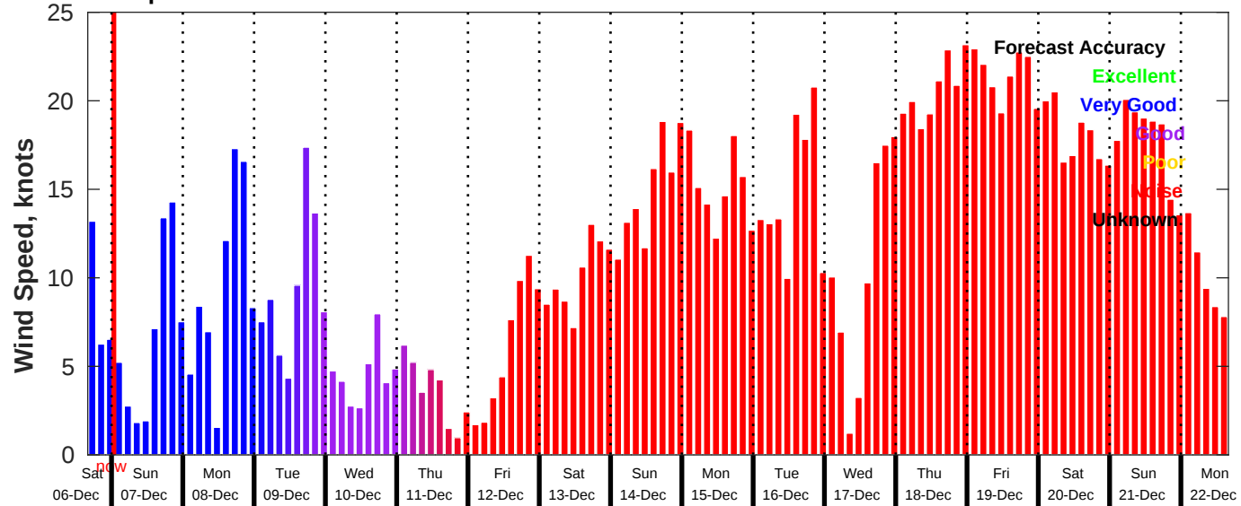
GFS Wind Speed Forecast for NDBC 46054 from 06-Dec-2025 16:00:00 to 22-Dec-2025 16:00:00
