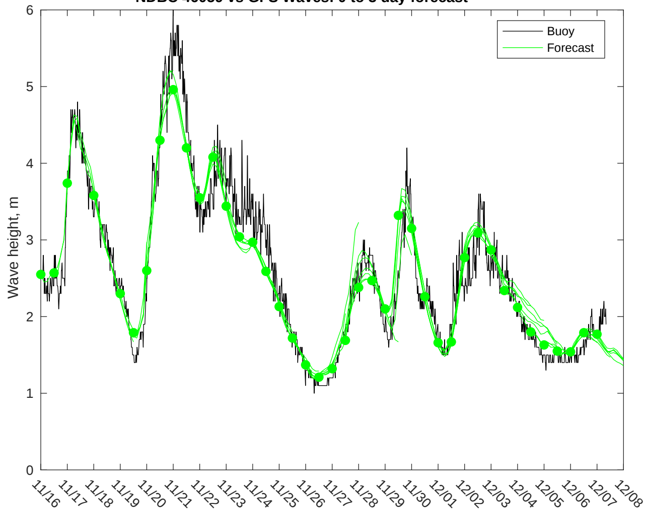
NDBC 46059 vs GFS Waves: 0 to 3 day forecast
