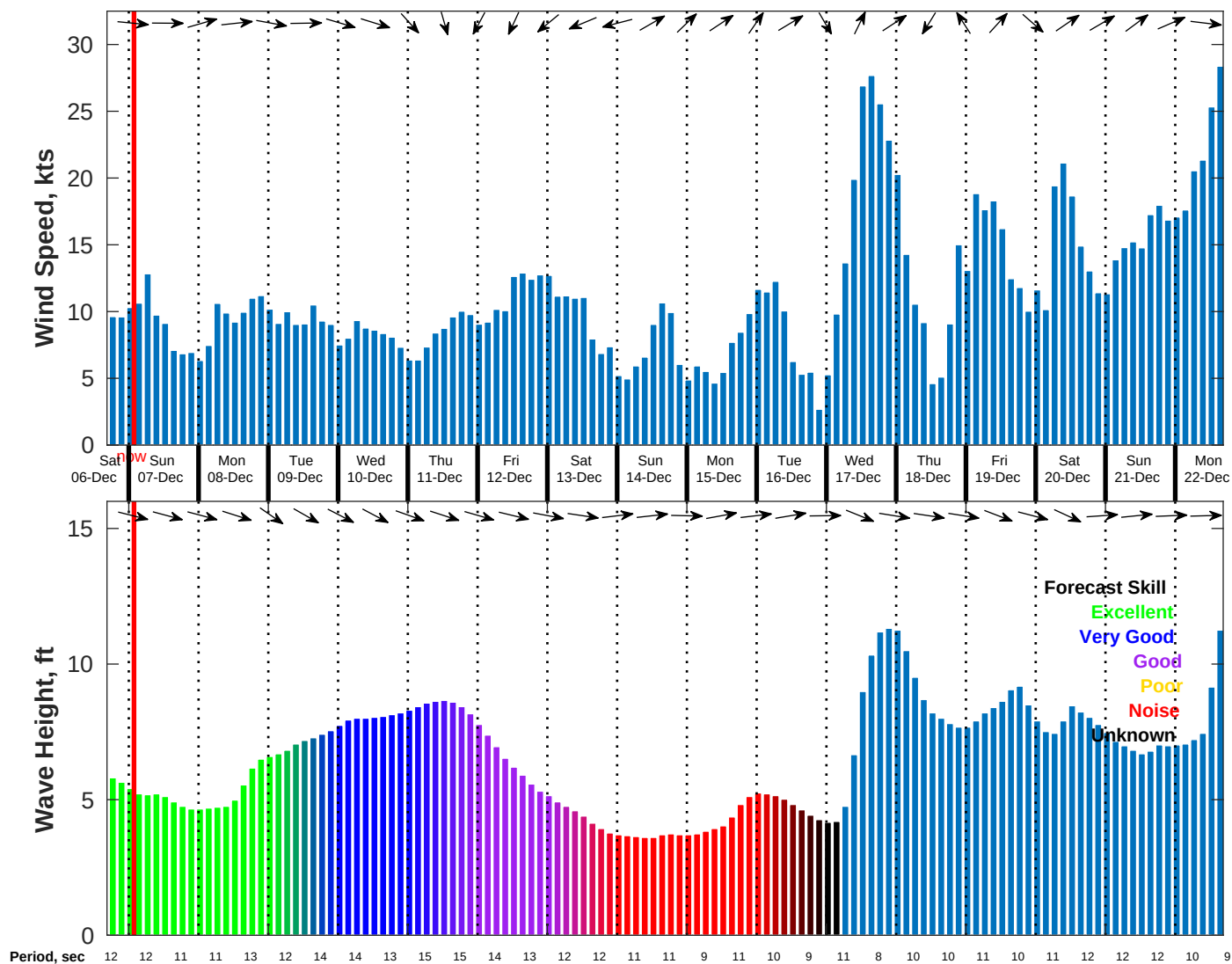
Wind & Wave Forecast for NDBC 46059 from 06-Dec-2025 17:00:00 to 22-Dec-2025 17:00:00
