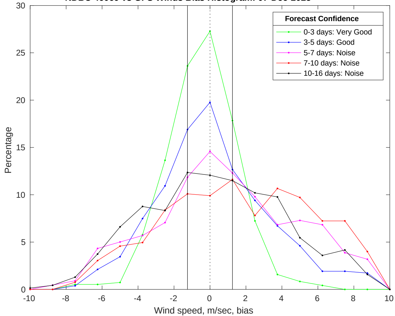
NDBC 46069 vs GFS Winds Bias Histogram: 07-Dec-2025
