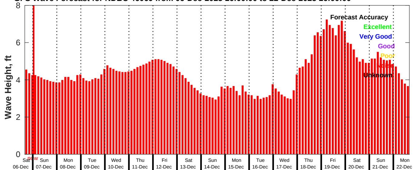
GFS Wave Forecast for NDBC 46069 from 06-Dec-2025 16:00:00 to 22-Dec-2025 16:00:00
