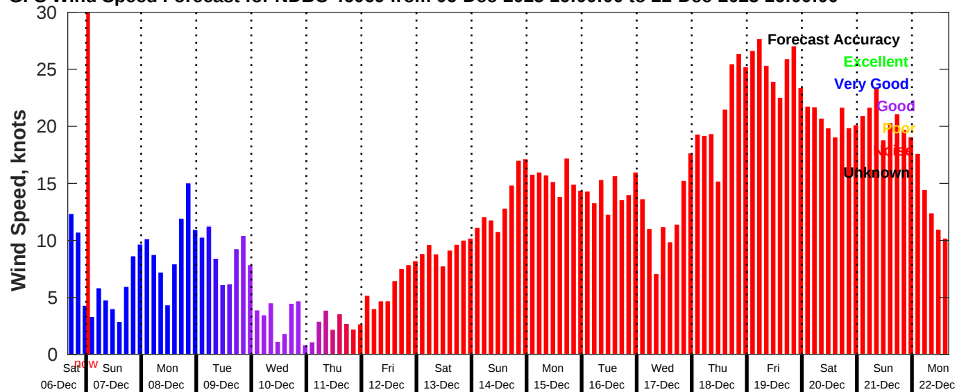
GFS Wind Speed Forecast for NDBC 46069 from 06-Dec-2025 16:00:00 to 22-Dec-2025 16:00:00
