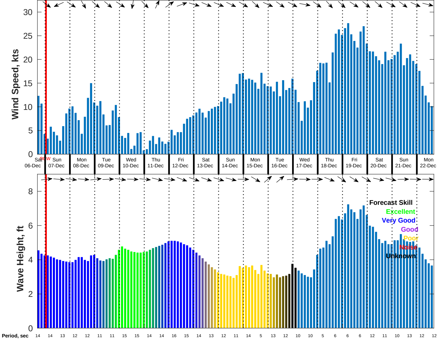
Wind & Wave Forecast for NDBC 46069 from 06-Dec-2025 16:00:00 to 22-Dec-2025 16:00:00
