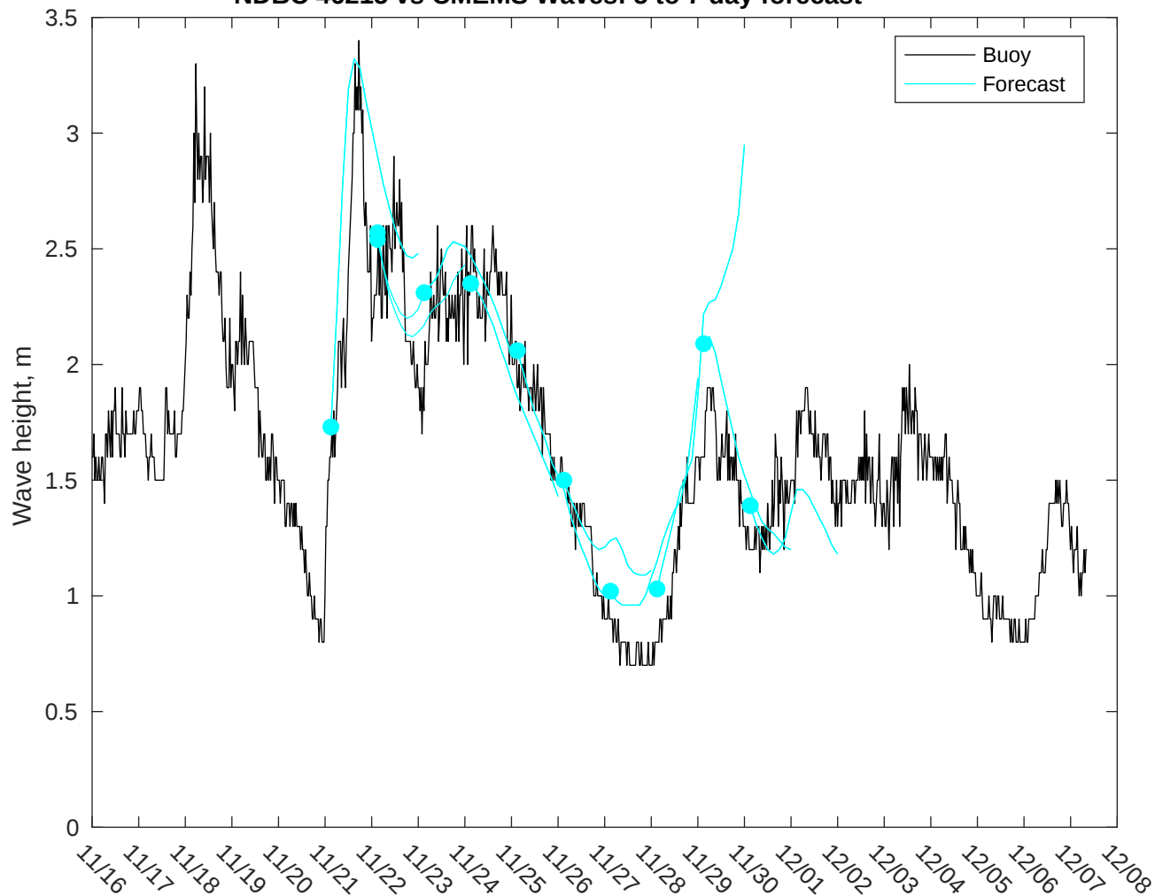
NDBC 46215 vs CMEMS Waves: 5 to 7 day forecast
