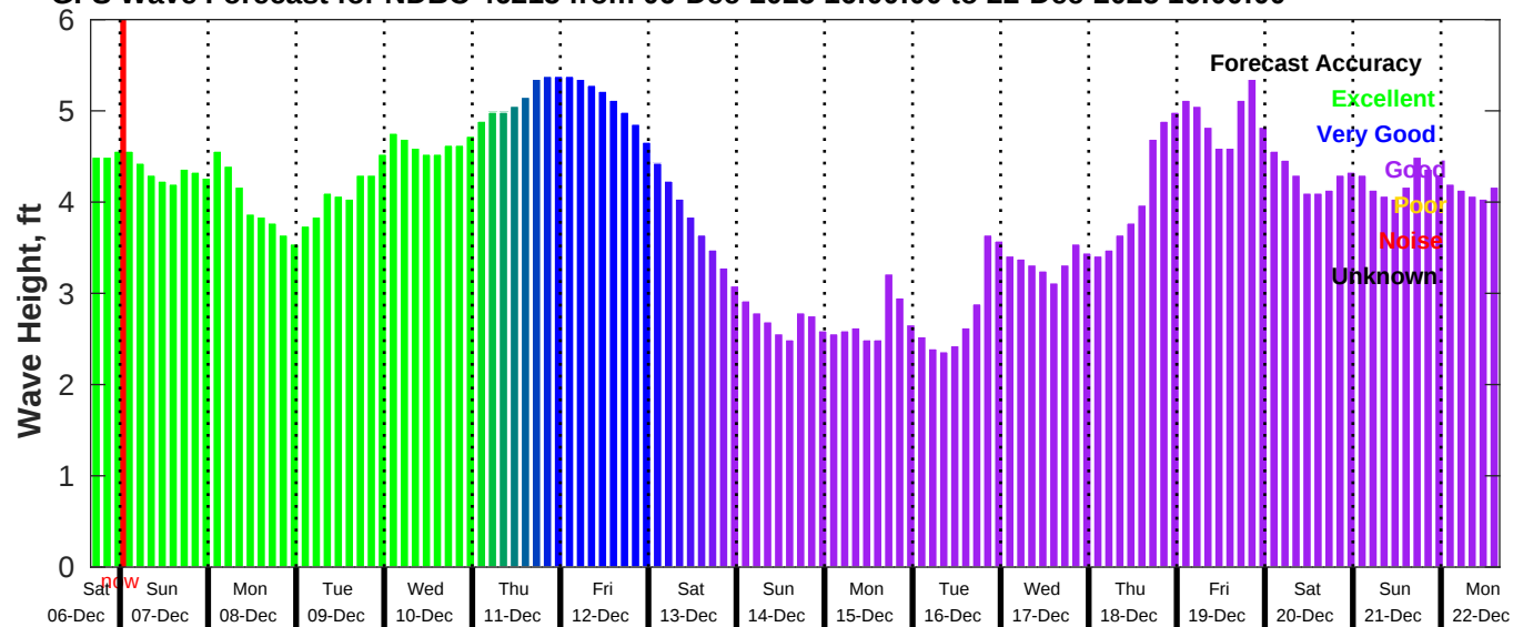
GFS Wave Forecast for NDBC 46215 from 06-Dec-2025 16:00:00 to 22-Dec-2025 16:00:00
