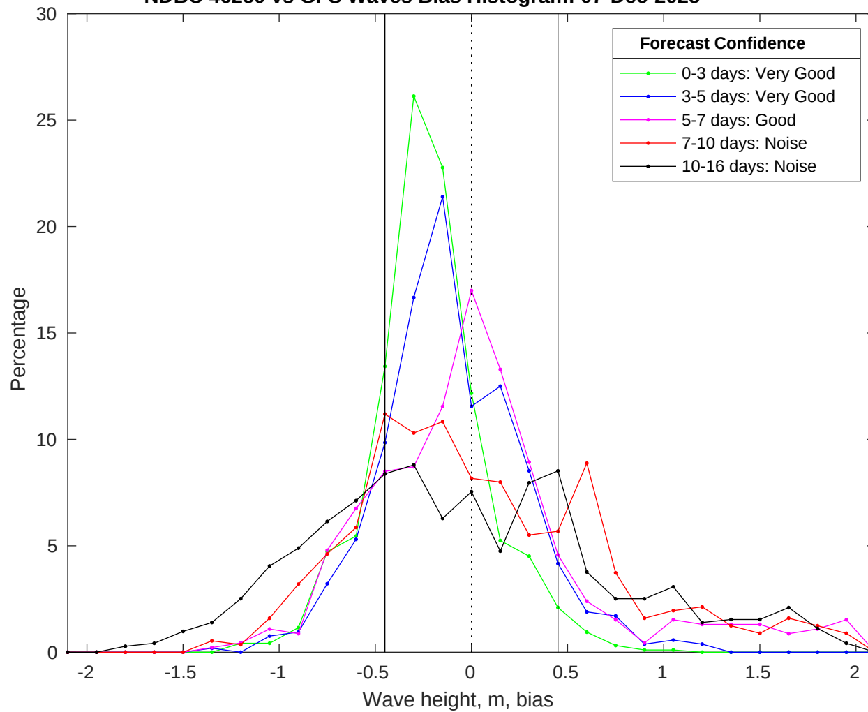
NDBC 46259 vs GFS Waves Bias Histogram: 07-Dec-2025
