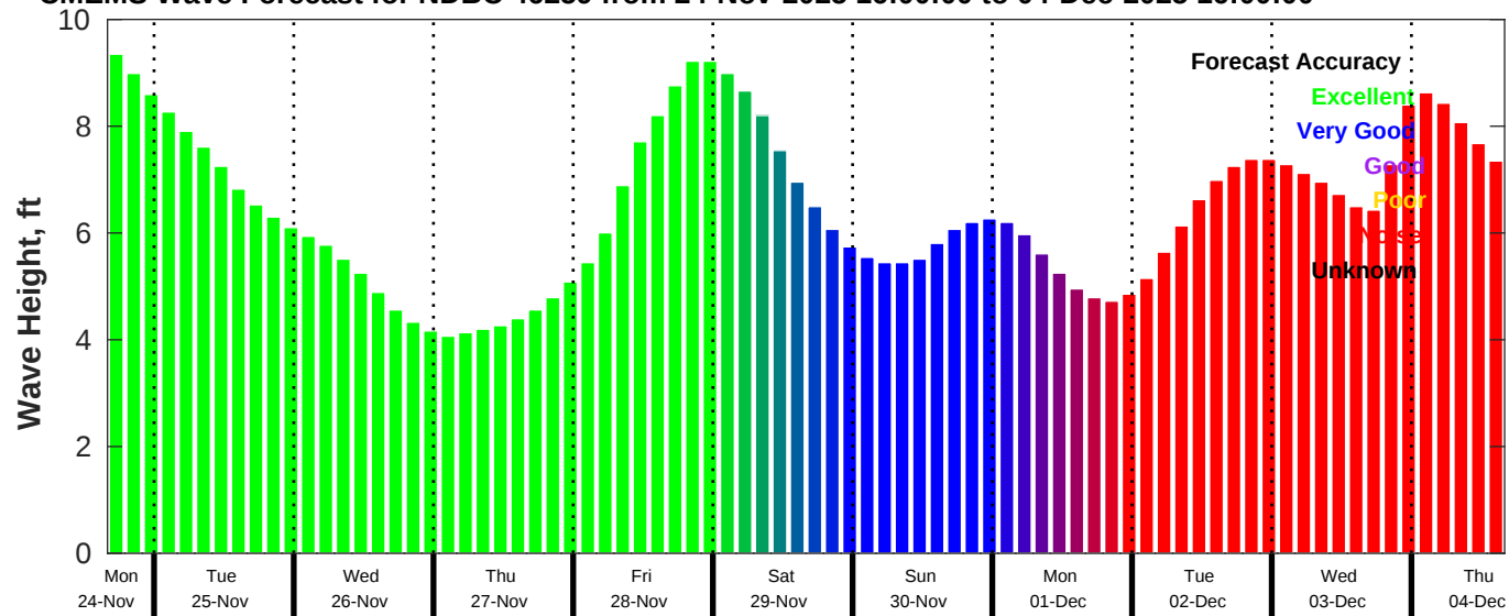
CMEMS Wave Forecast for NDBC 46259 from 24-Nov-2025 16:00:00 to 04-Dec-2025 16:00:00
