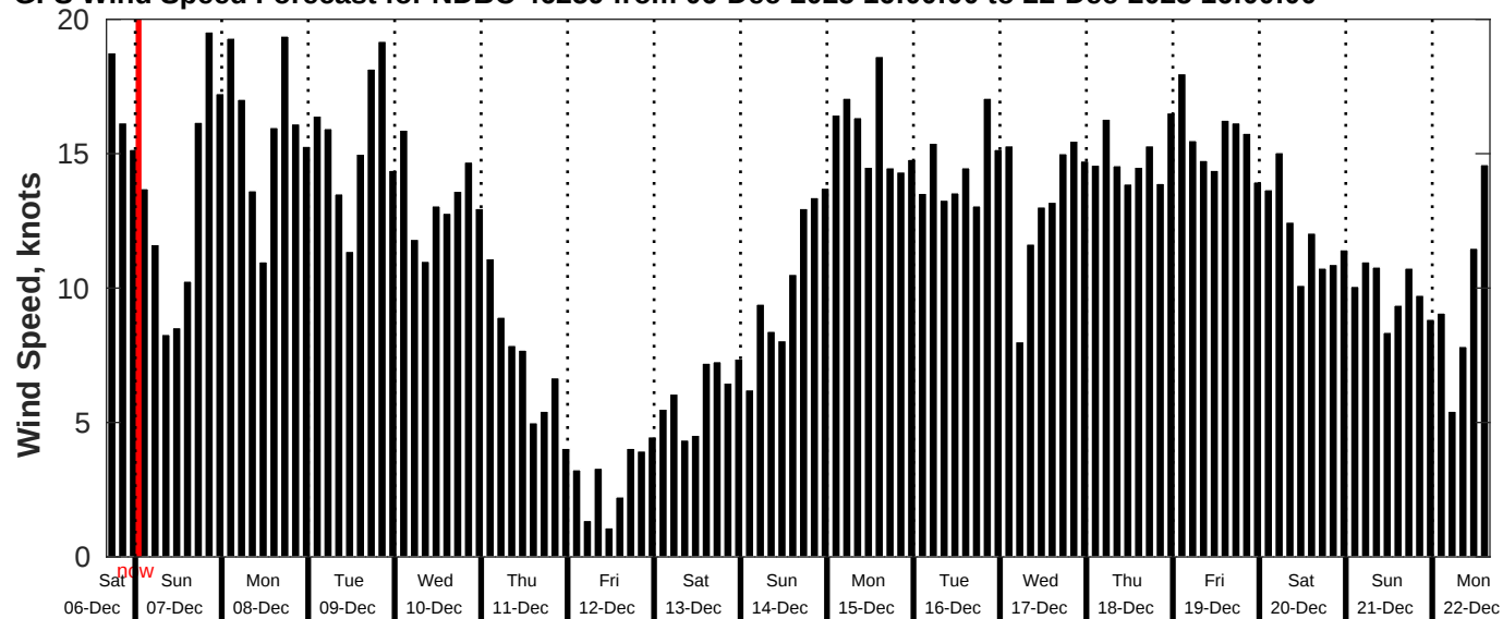
GFS Wind Speed Forecast for NDBC 46259 from 06-Dec-2025 16:00:00 to 22-Dec-2025 16:00:00
