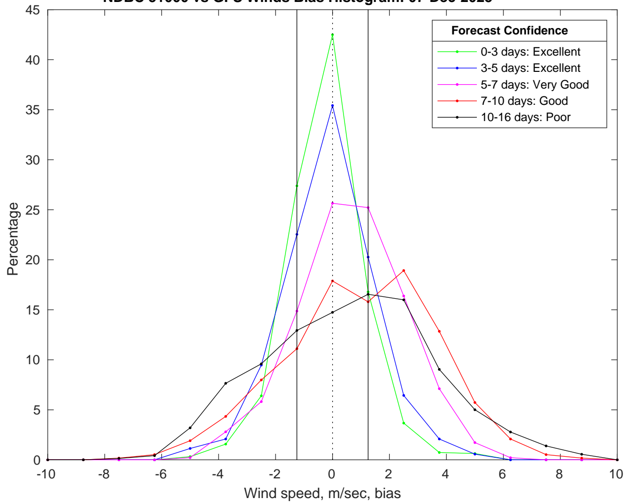
NDBC 51000 vs GFS Winds Bias Histogram: 07-Dec-2025
