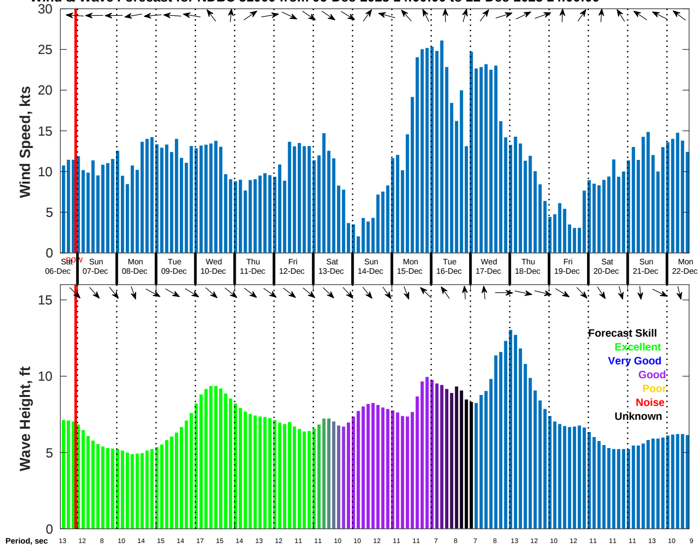
Wind & Wave Forecast for NDBC 51000 from 06-Dec-2025 14:00:00 to 22-Dec-2025 14:00:00
