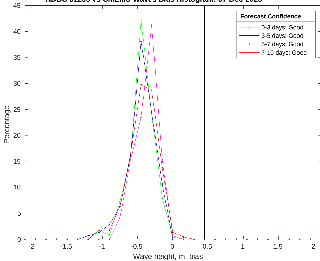
NDBC 51209 vs CMEMS Waves Bias Histogram: 07-Dec-2025
