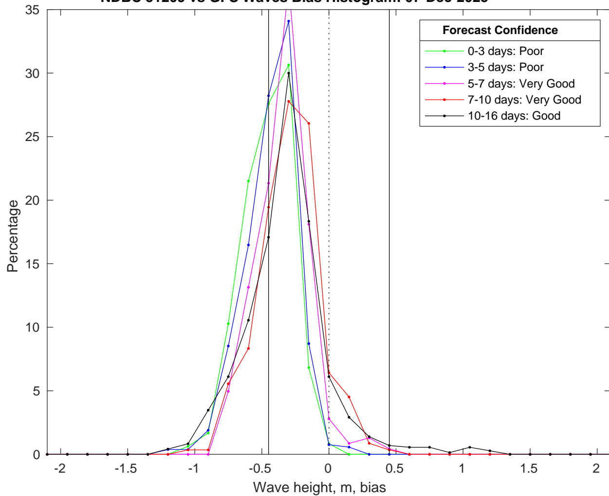
NDBC 51209 vs GFS Waves Bias Histogram: 07-Dec-2025
