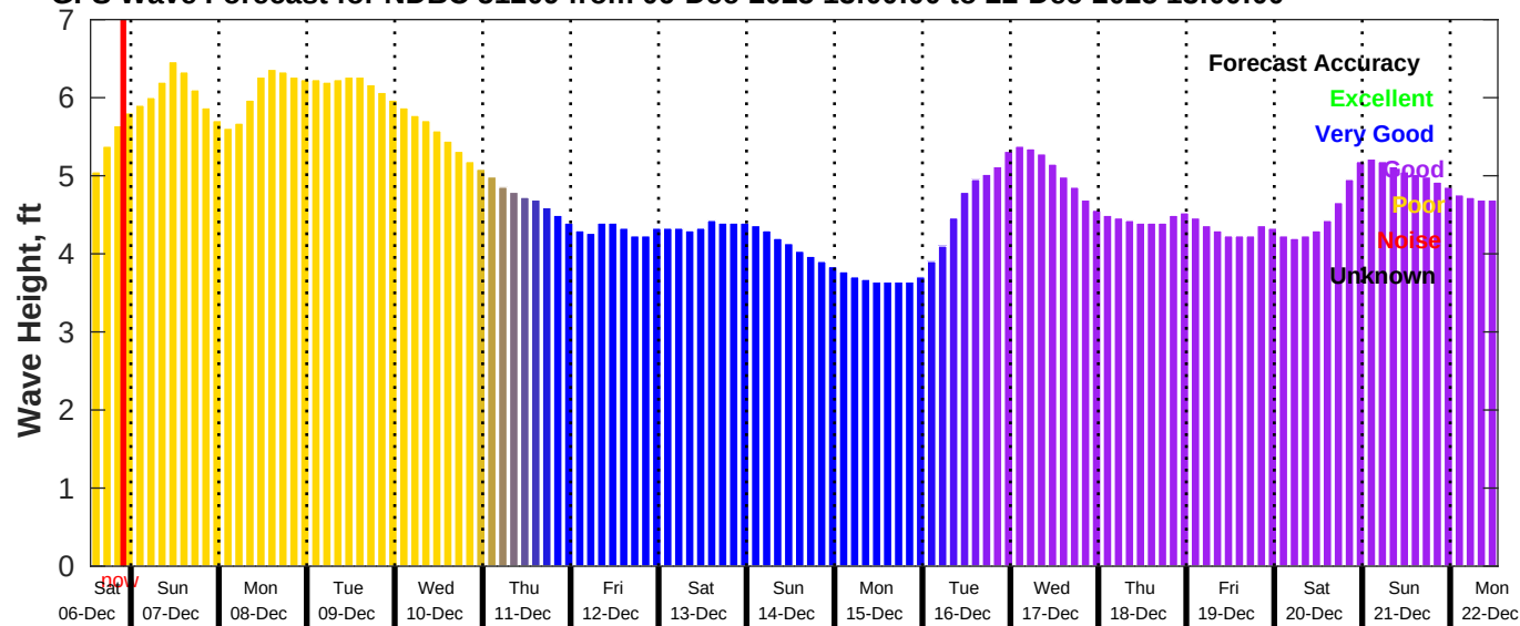
GFS Wave Forecast for NDBC 51209 from 06-Dec-2025 13:00:00 to 22-Dec-2025 13:00:00
