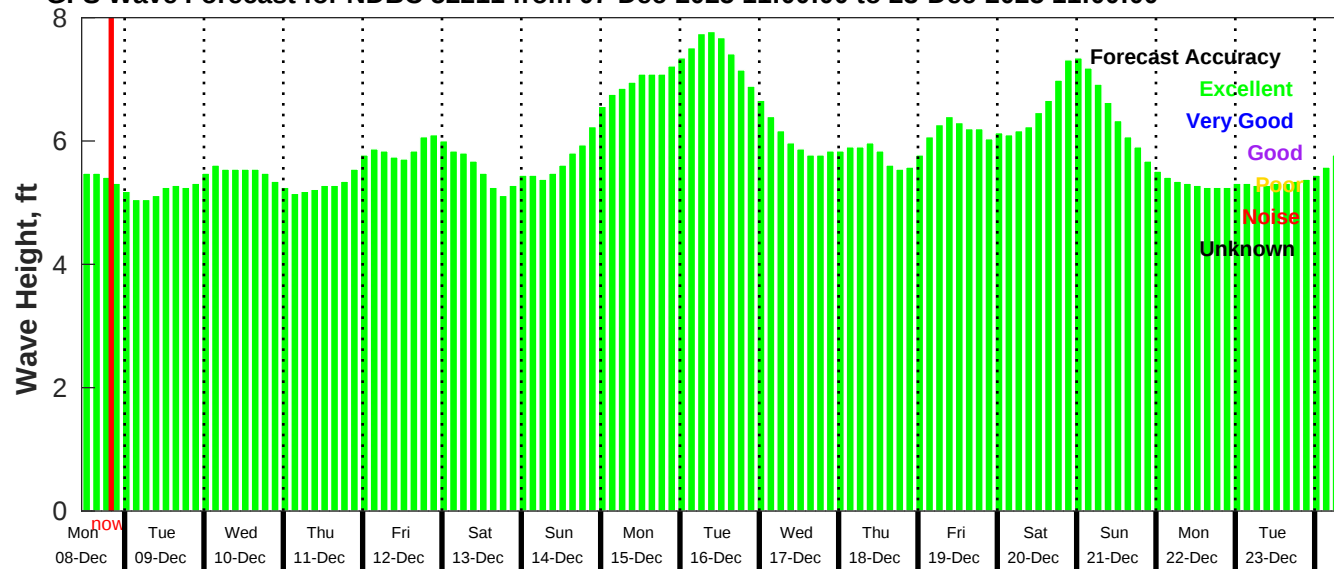
GFS Wave Forecast for NDBC 52211 from 07-Dec-2025 11:00:00 to 23-Dec-2025 11:00:00
