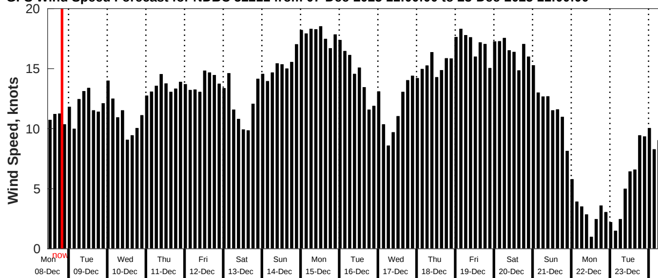
GFS Wind Speed Forecast for NDBC 52211 from 07-Dec-2025 11:00:00 to 23-Dec-2025 11:00:00
