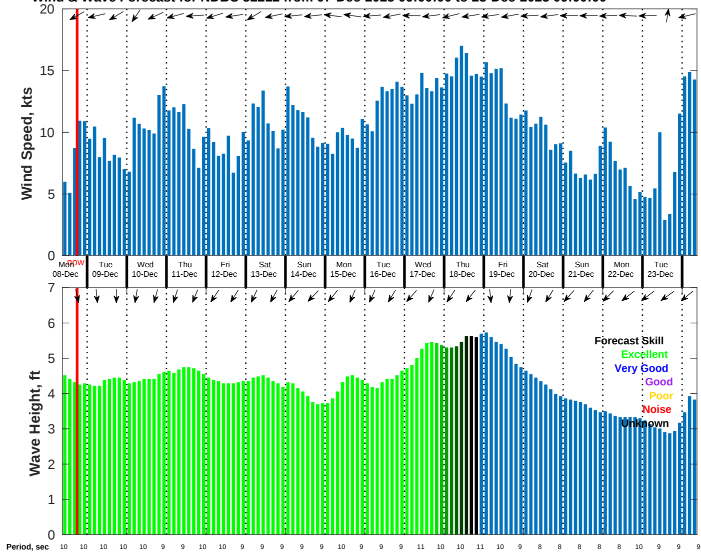
Wind & Wave Forecast for NDBC 52212 from 07-Dec-2025 09:00:00 to 23-Dec-2025 09:00:00
