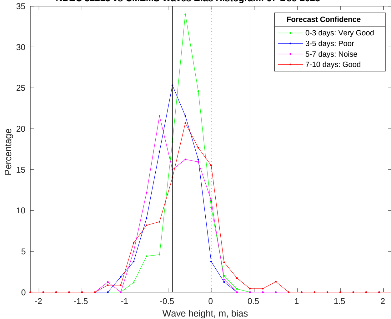
NDBC 52213 vs CMEMS Waves Bias Histogram: 07-Dec-2025
