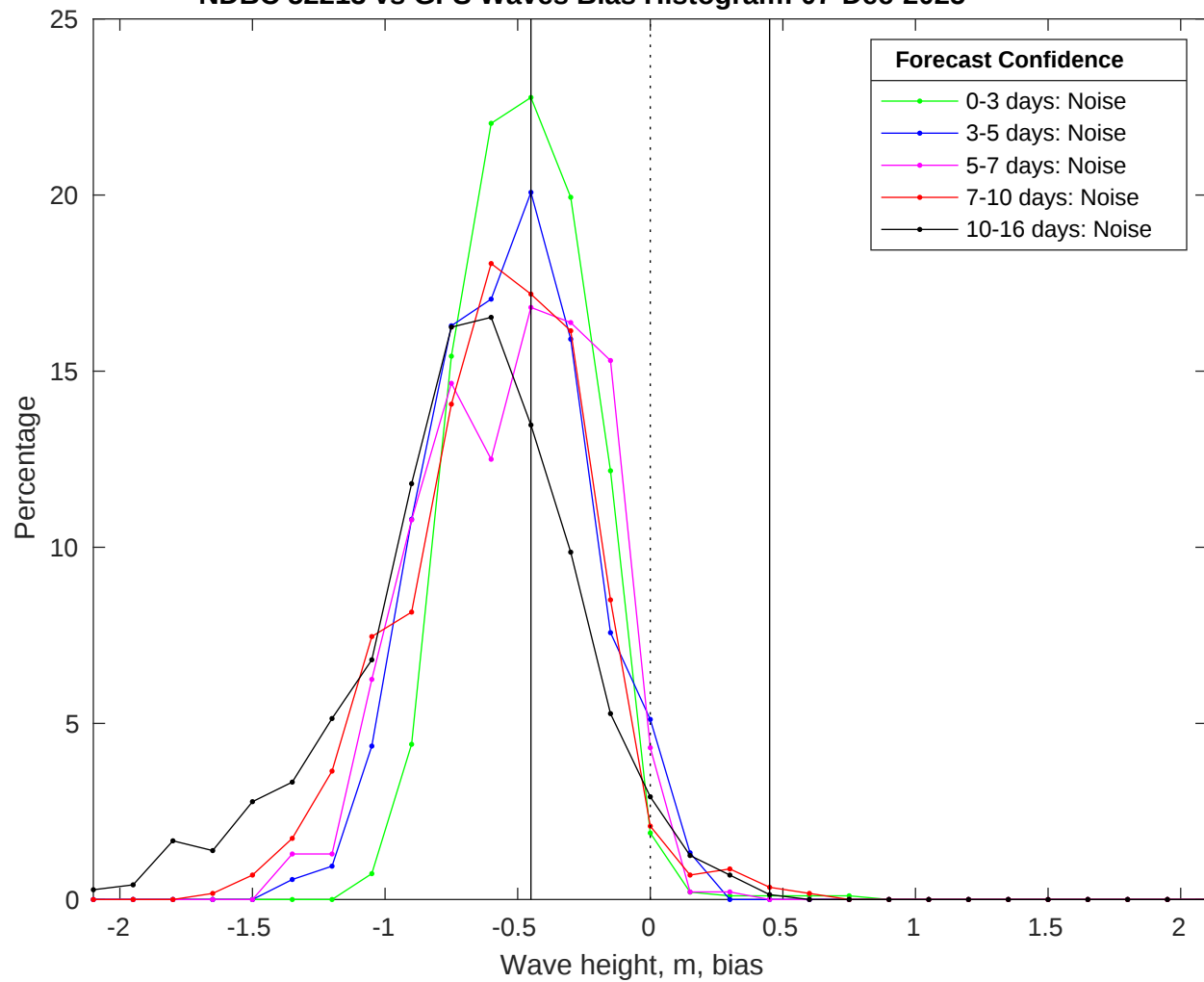
NDBC 52213 vs GFS Waves Bias Histogram: 07-Dec-2025
