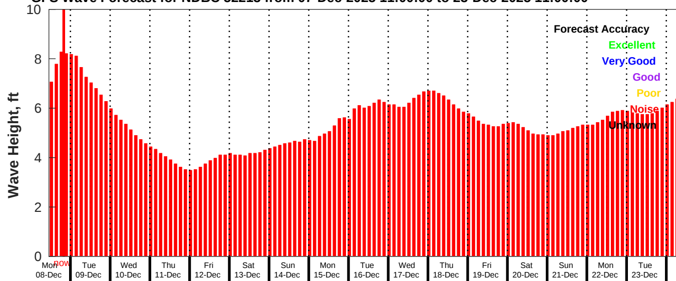
GFS Wave Forecast for NDBC 52213 from 07-Dec-2025 11:00:00 to 23-Dec-2025 11:00:00
