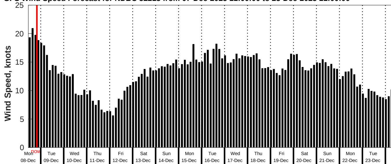
GFS Wind Speed Forecast for NDBC 52213 from 07-Dec-2025 11:00:00 to 23-Dec-2025 11:00:00
