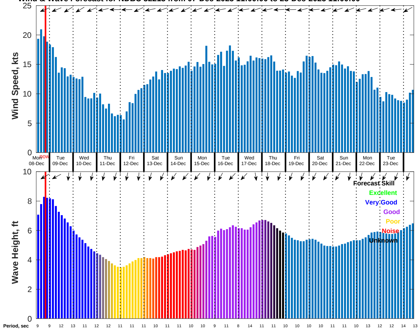
Wind & Wave Forecast for NDBC 52213 from 07-Dec-2025 11:00:00 to 23-Dec-2025 11:00:00
